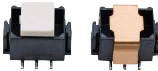
Left = New plastic cap, Right = Previous metal cap
